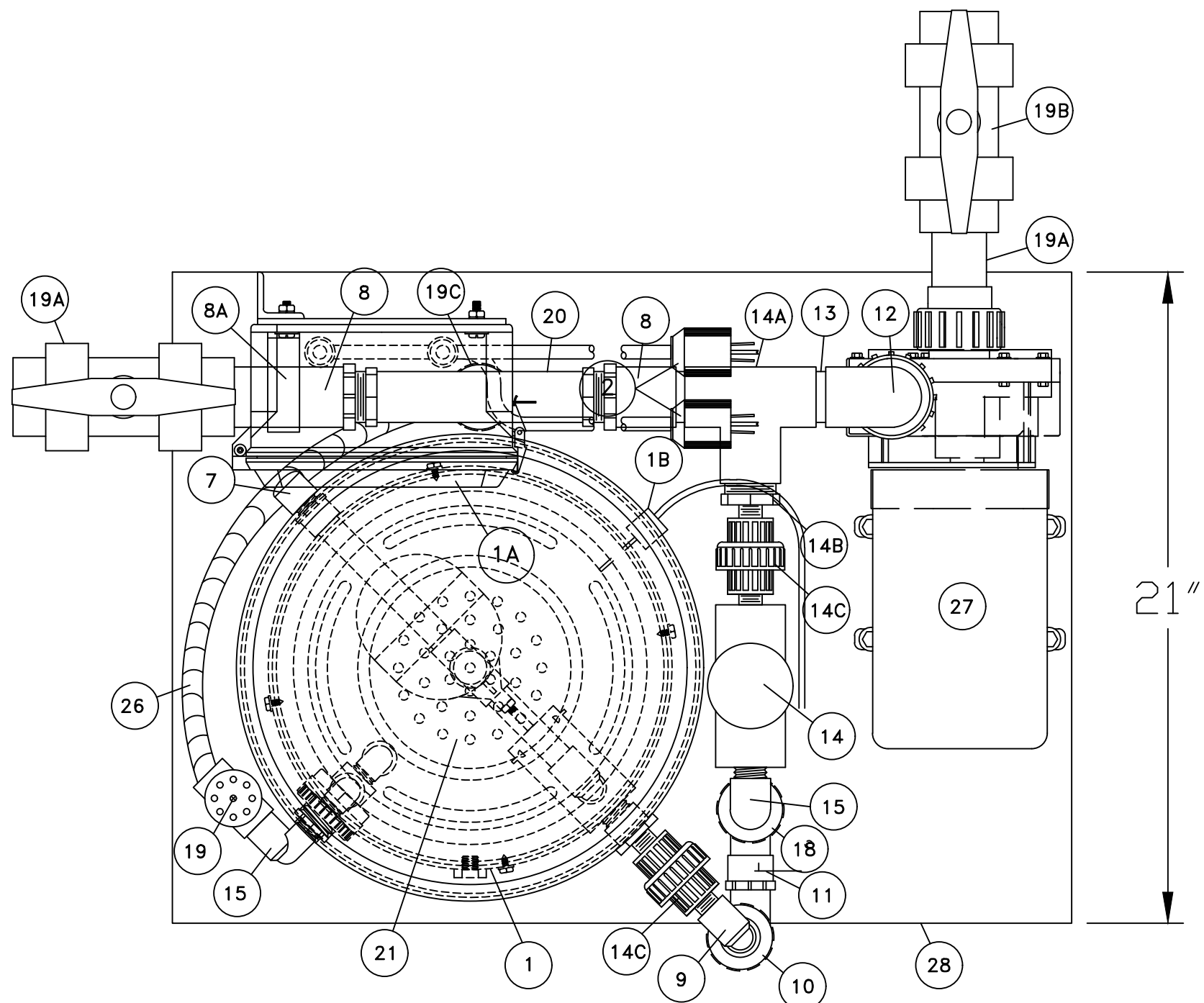
SYSTEM PLAN
