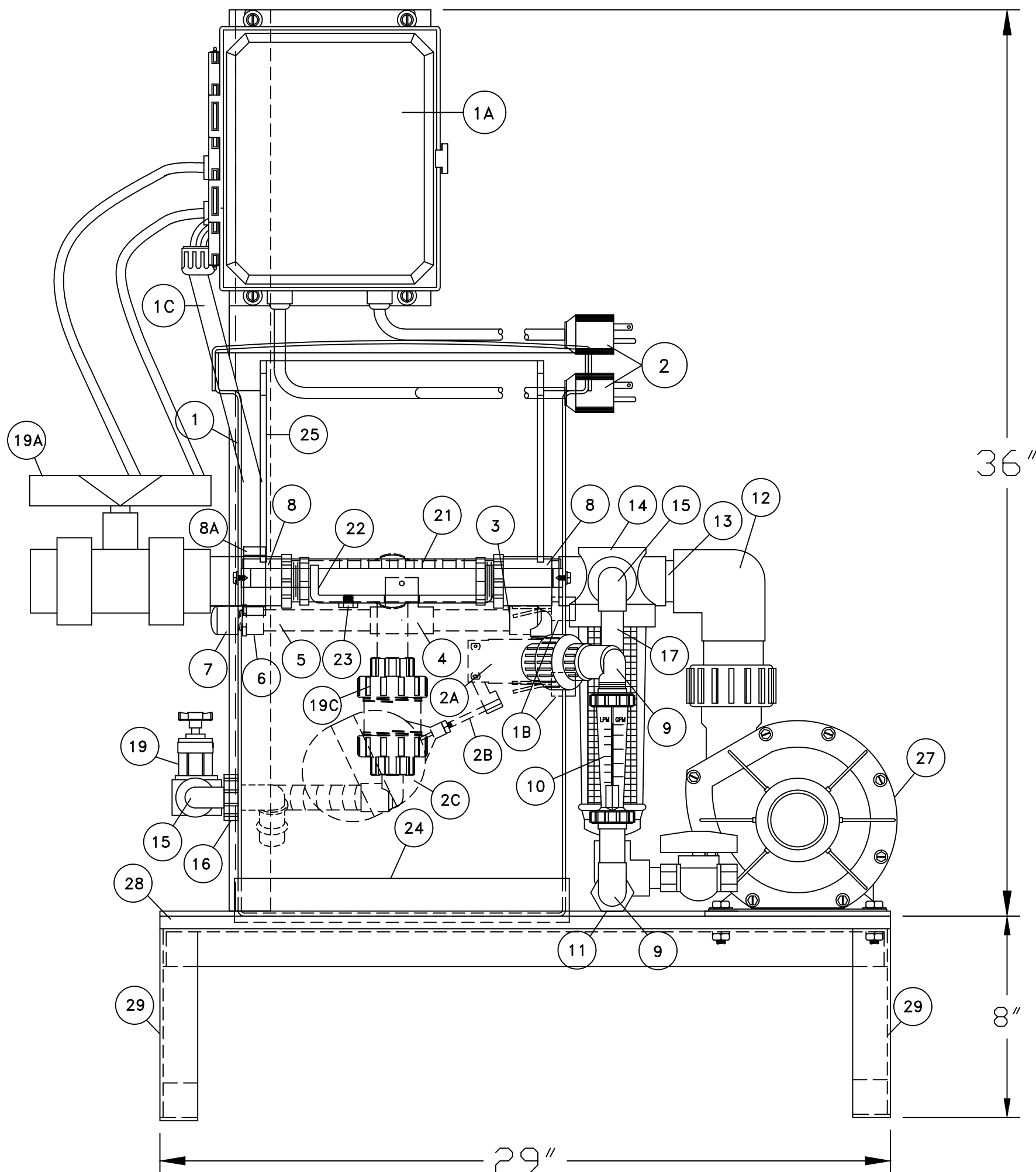
SYSTEM ELEVATION
