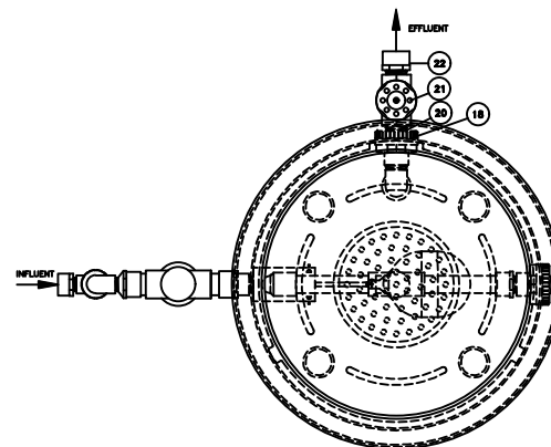
SYSTEM PLAN
