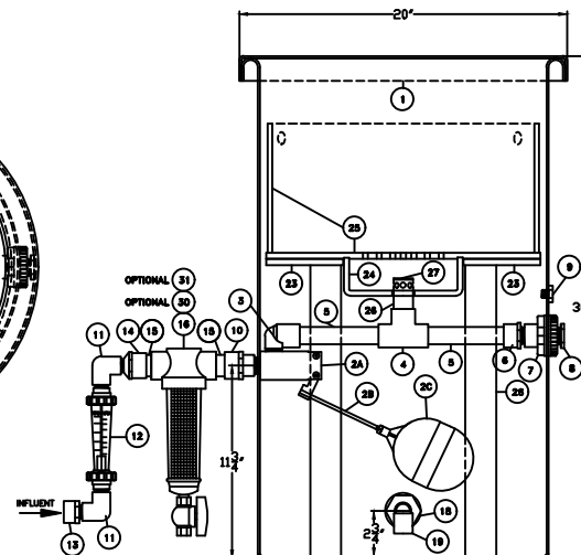
SYSTEM ELEVATION
