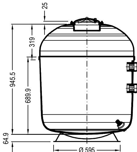
SECTION A
